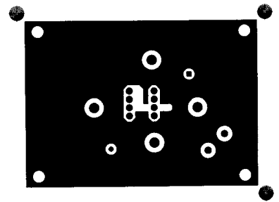
FIGURE 1C. BOTTOM LAYOUT
