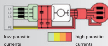
Topology of parasitic currents
