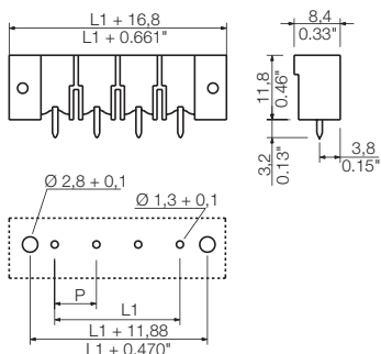
Dimensioned drawing
