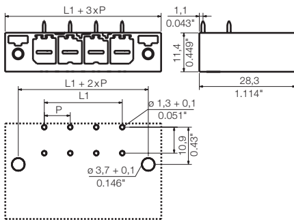
Dimensioned drawing
