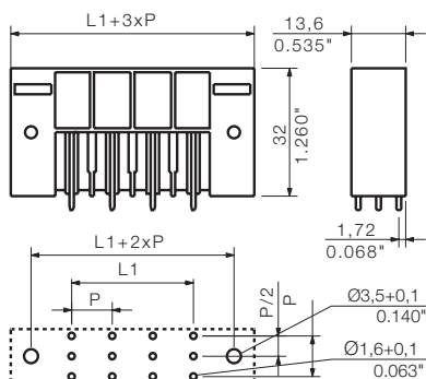
Dimensioned drawing
