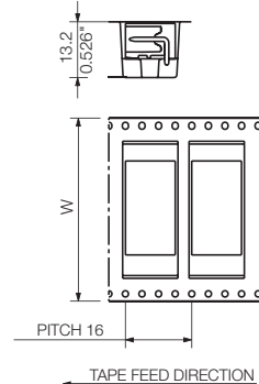
Dimensioned drawing
