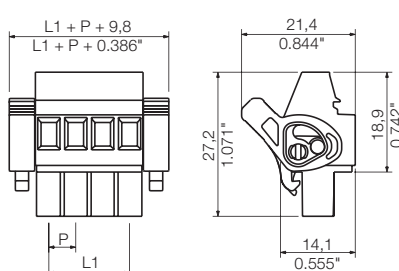
Dimensioned drawing
