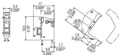
Version left
