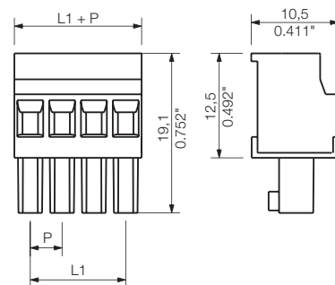
Dimensioned drawing
