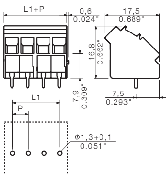
Dimensioned drawing
