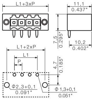
Dimensioned drawing
