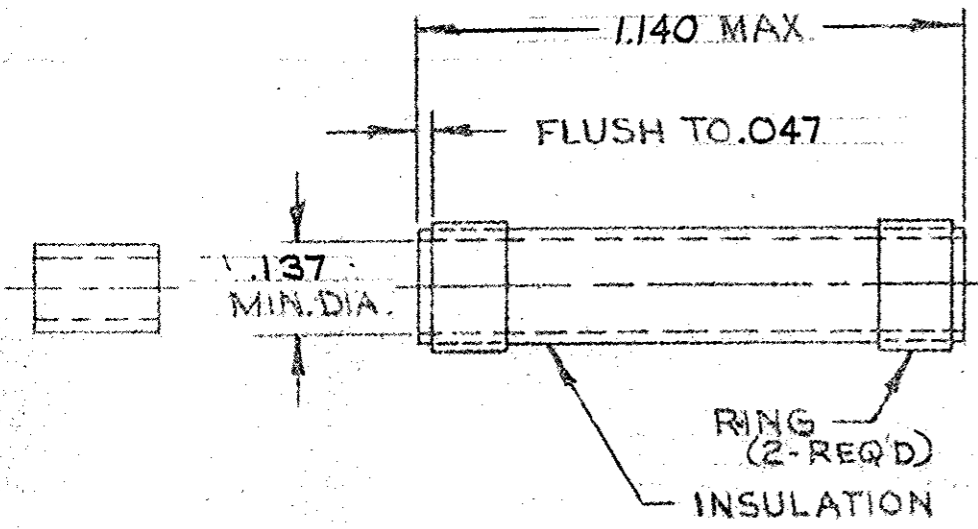
BUSHING
